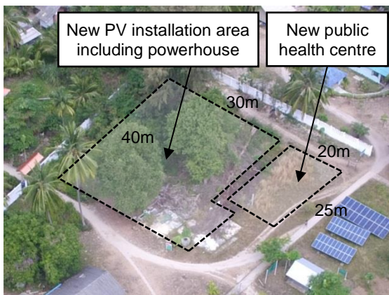
Figure 35: Possible area to install new powerhouse and PV
