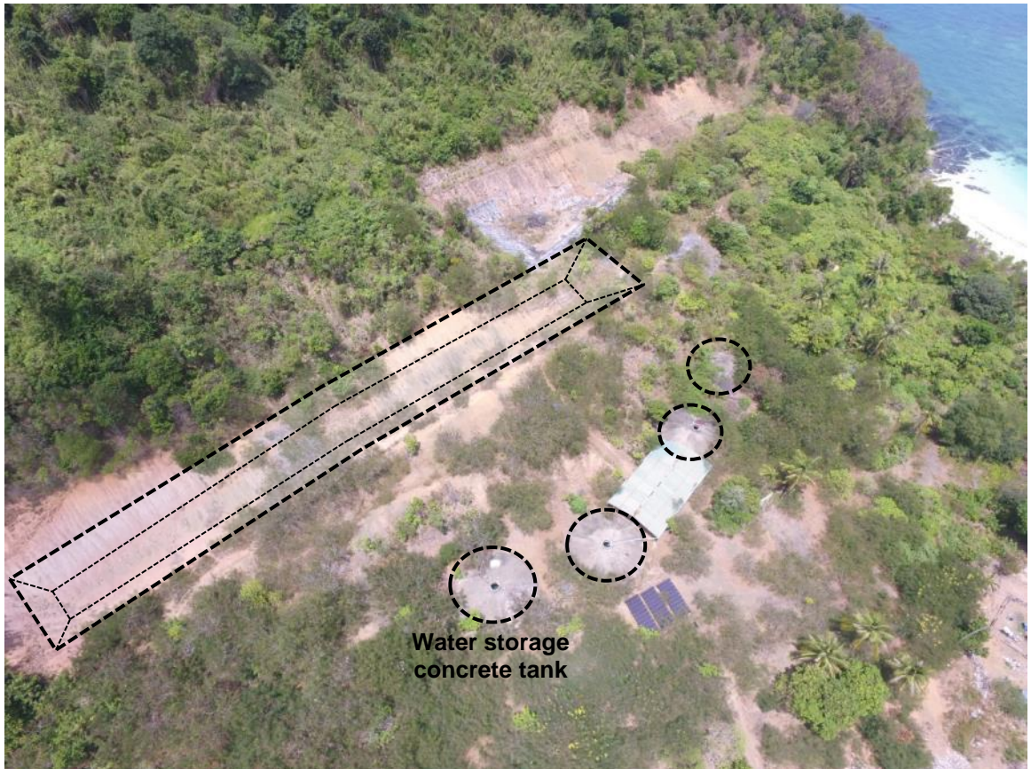
Figure 45: Overview of water system and storage
